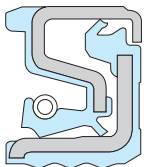
Simmerring® Cassette seal type 1
